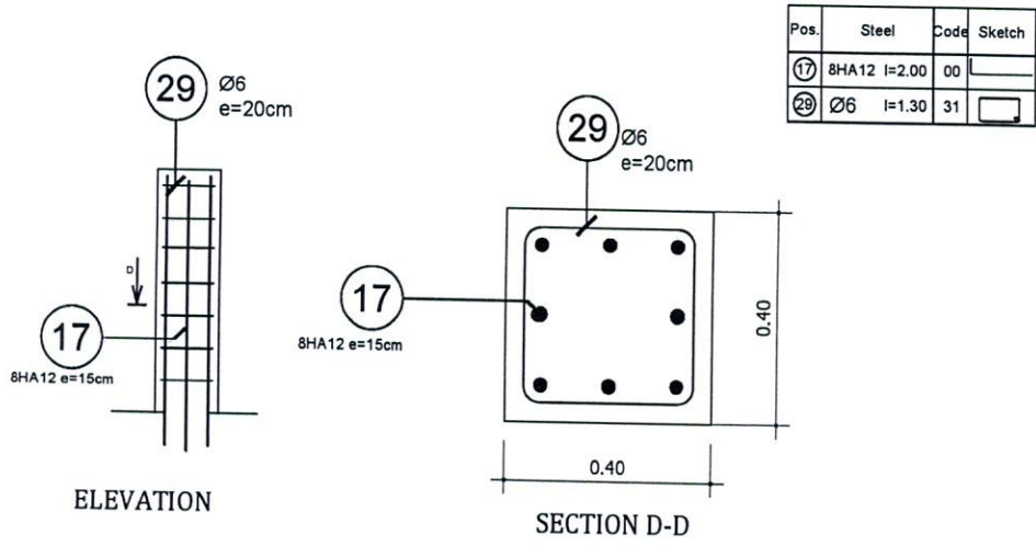
SIGNALIZATION COLUMN 0.40X0.40 OF THE BRIDGE (4)
