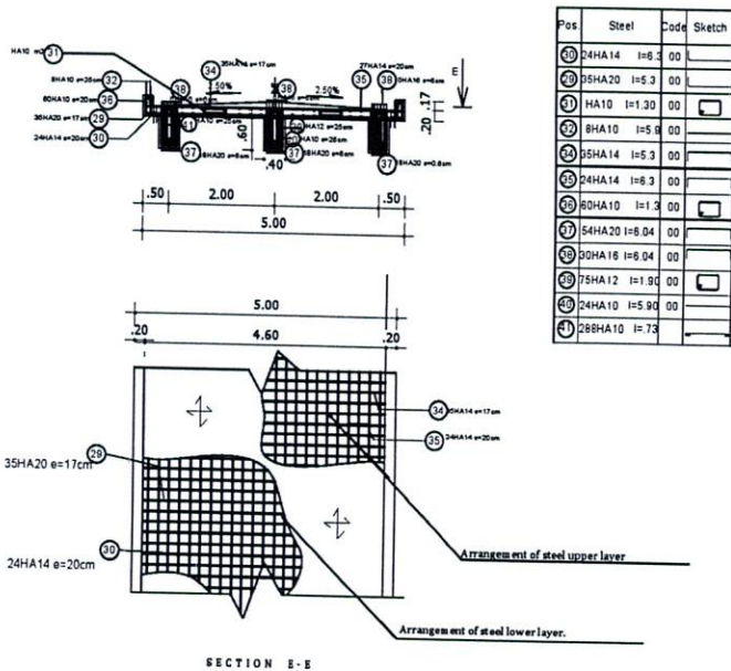
DETAILS ON DECK SLAB
