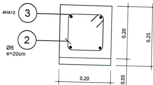
SECTION G-G
