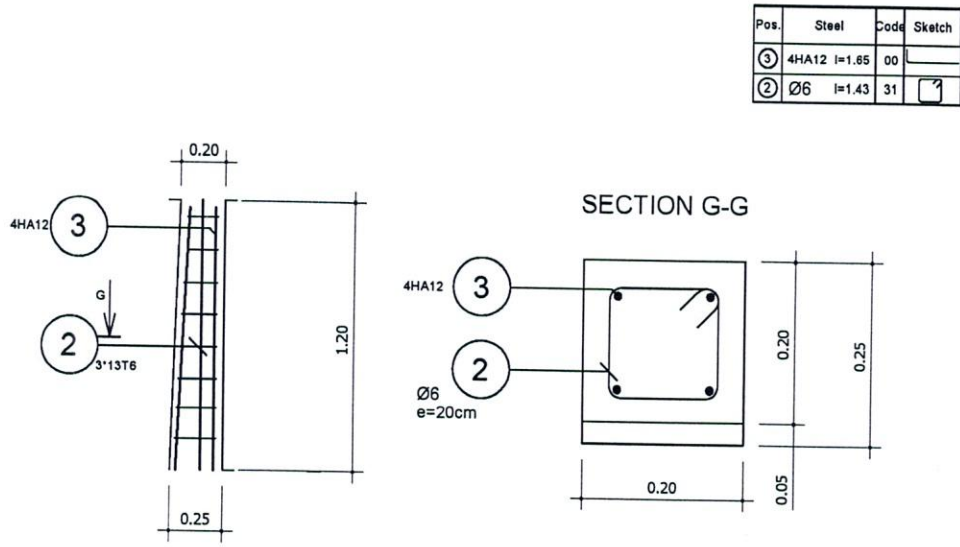
Column of height 1.20m guard rail
