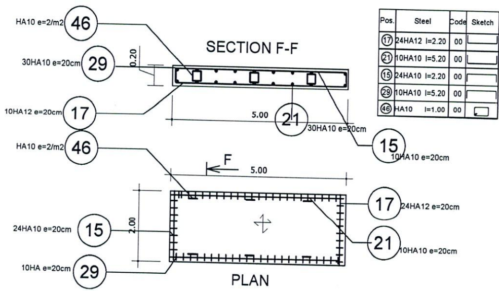
DETAIL C ( DALLE DE TRANSITION ) (2)
