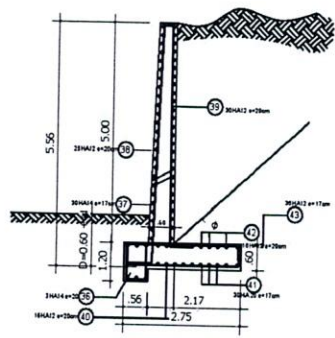
SECTION G-G
