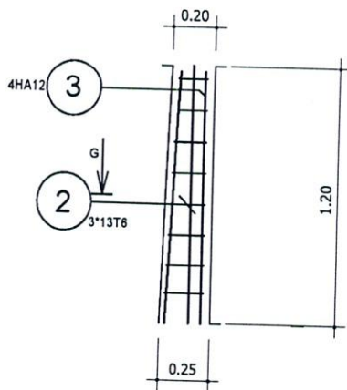
Column of height 1.20m guard rail
