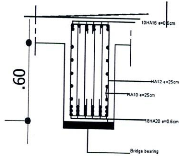
DETAIL MAIN BEAM
