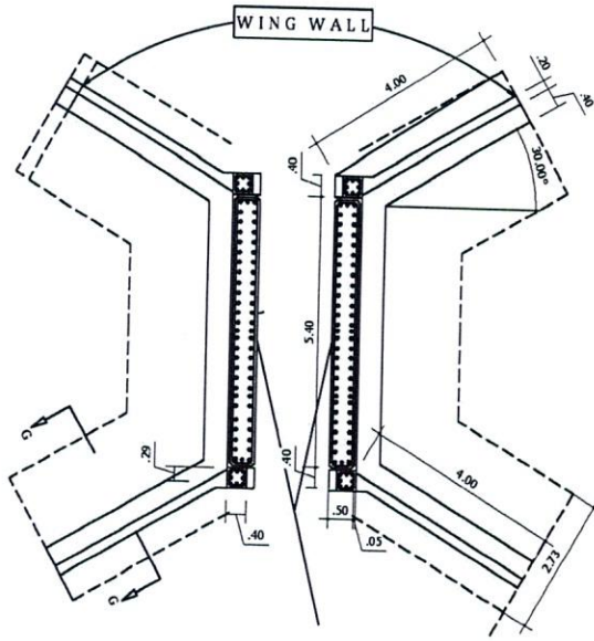
ABUTMENT AND WING WALL
